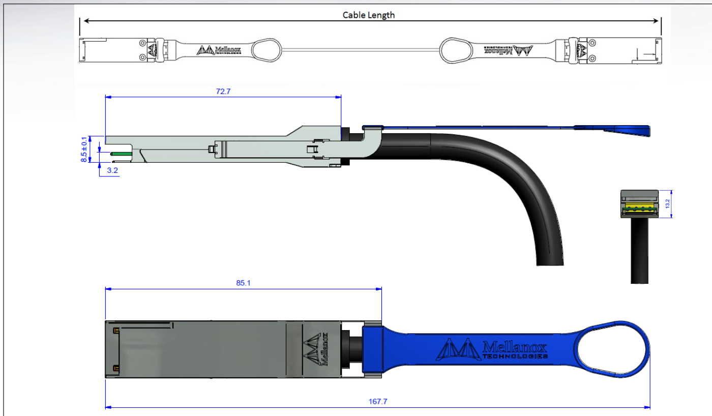
Figure 1. Mechanical Drawings and Information
