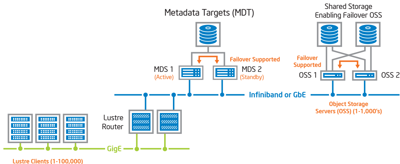
Figure 2. Typical Lustre configuration
